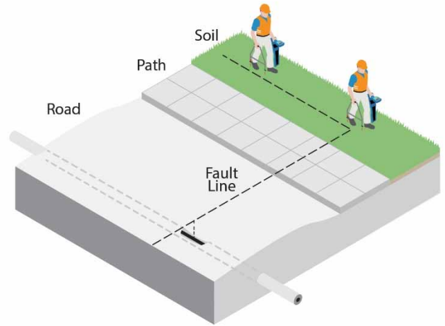
Figure 9.2: Locating faults with the locator and A-frame
