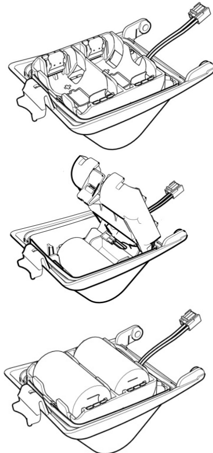
Figure 4.7 Locator D-cell holder
