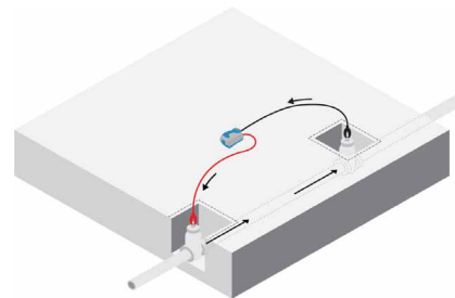
Figure 8.5: Making double-ended connections
