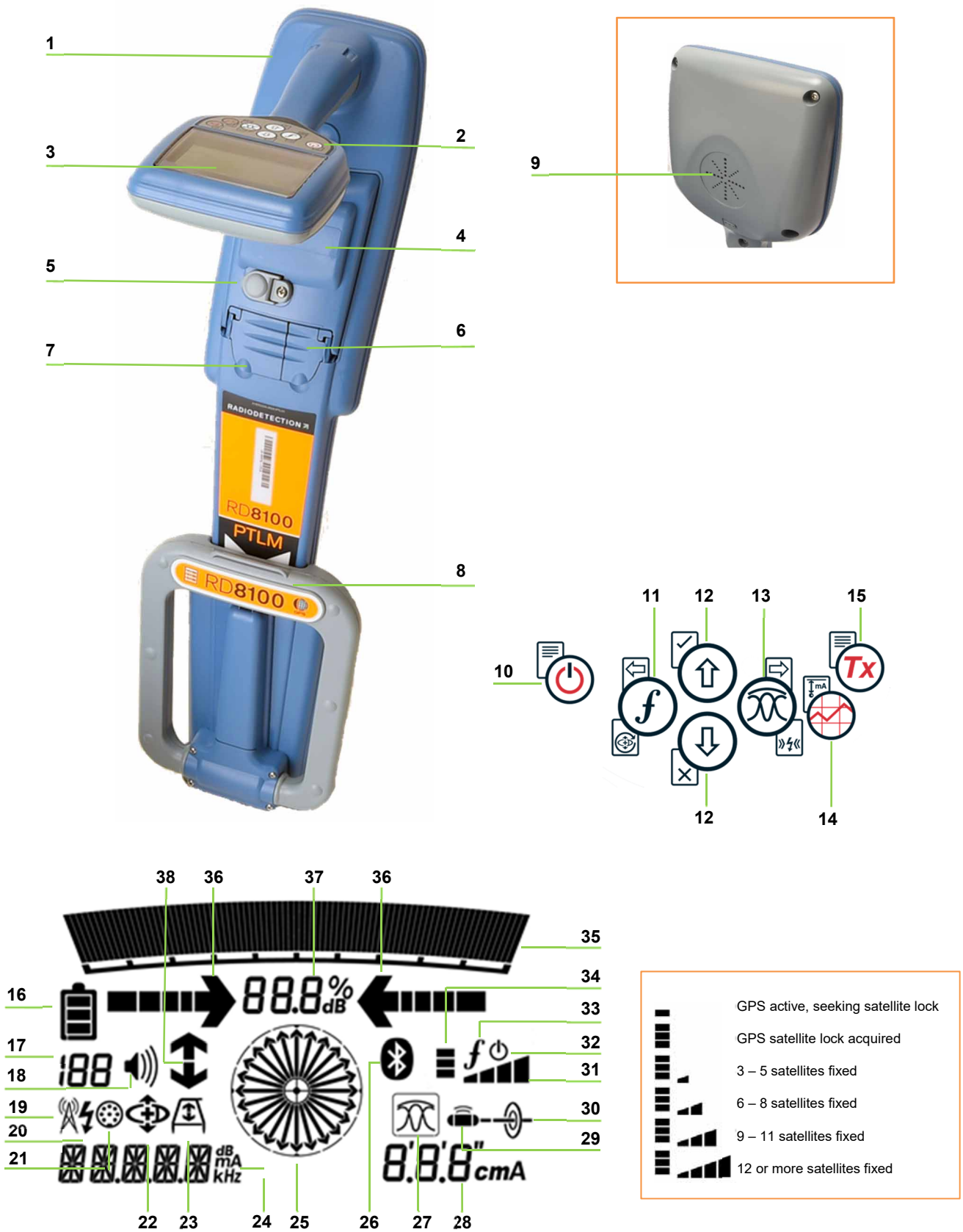
Figure 3.1 RD8100 cable, pipe and marker locator
