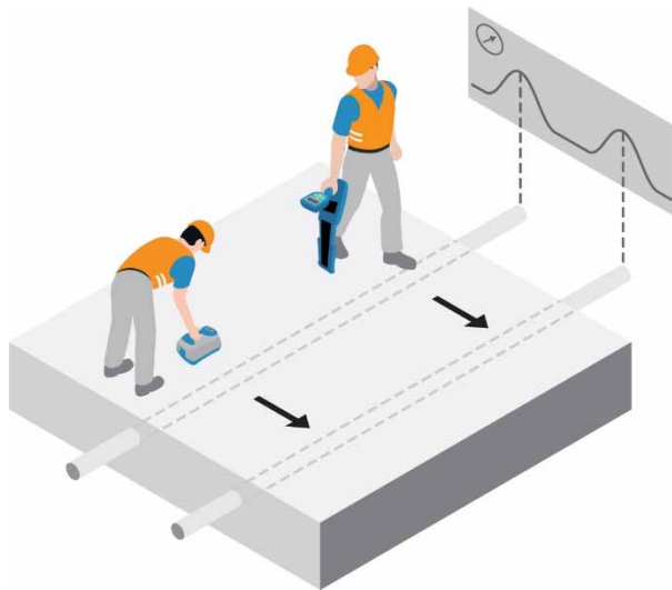
Figure 5.9: Inductive search
