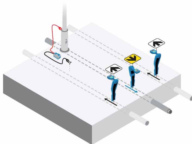
Figure 10.1: Current Direction
