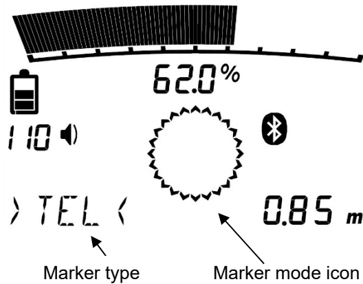
Figure 6.1 Marker mode
