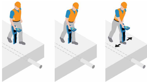
Figure 5.6: Pinpointing a target line
