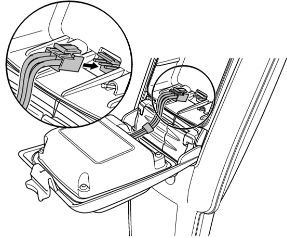
Figure 4.2 Li-ion battery pack connection
