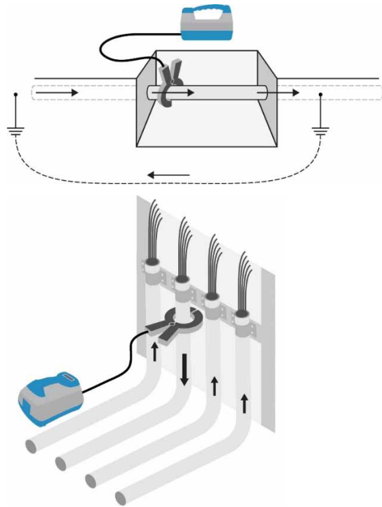
Figures 14.5 – 14.6: Connecting transmitter clamps
