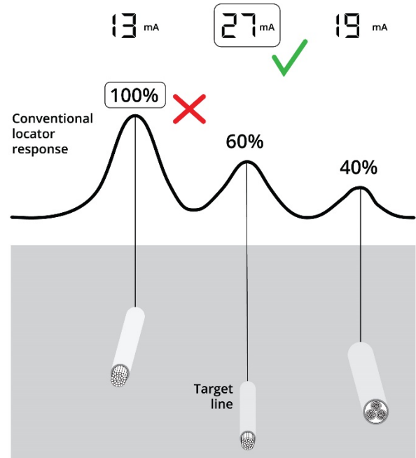
Figures 7.4 – 7.6 Taking current readings
