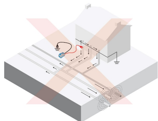
Figures 8.1 – 8.4: Nulling utilities & interference from services
