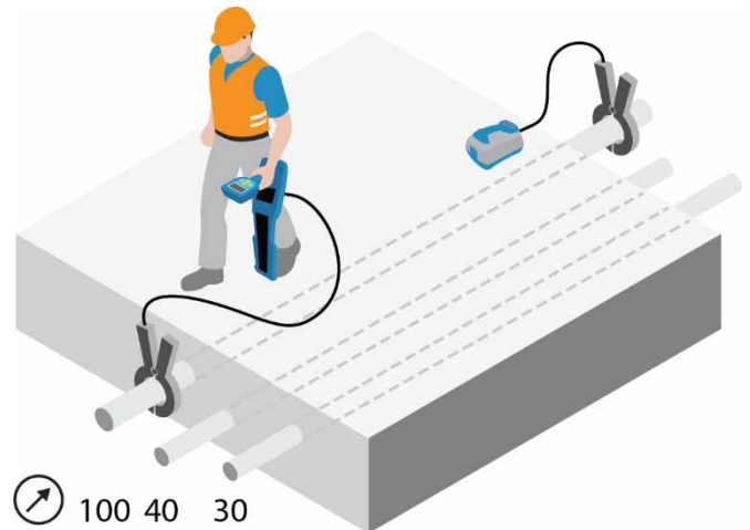
Figure 14.1: Connecting clamps
