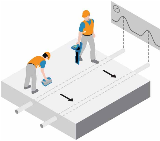
Figure 5.6 Nulling Out - Single person sweep
