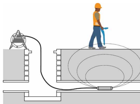
Figure 14.8 Sonde deployment
