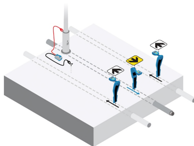
Figure 11.1: Current Direction
