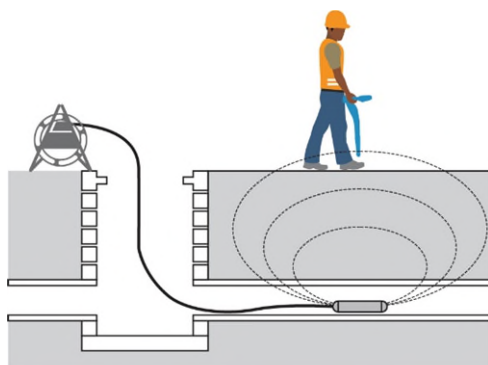
Figure 15.8 Sonde deployment
