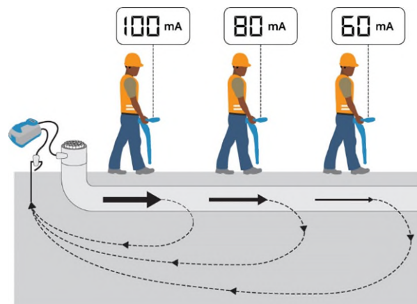
Figure 8.7: Current readings using transmitter signals
