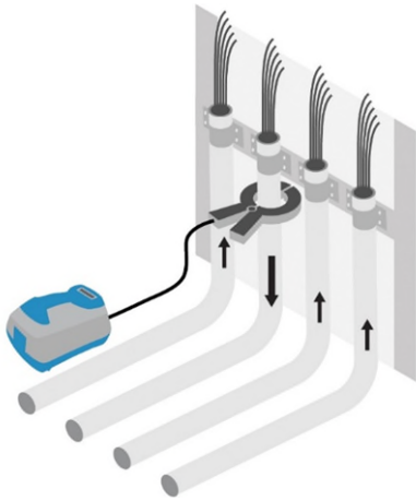
Figures 15.5 – 15.6: Connecting transmitter clamps
