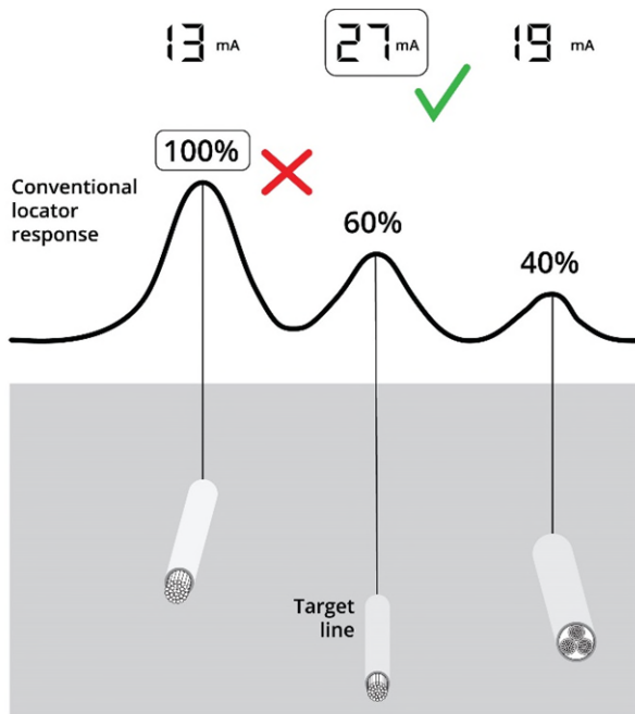
Figures 8.4 – 8.6 Taking current readings
