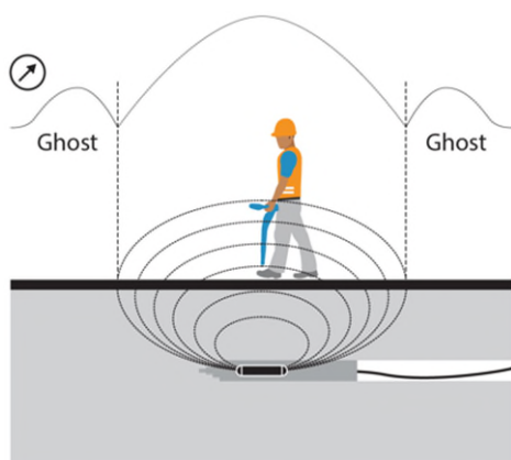
Figure 15.9 Locating a sonde
