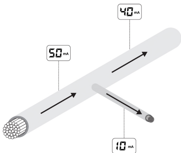
Figure 8.3 Current readings
