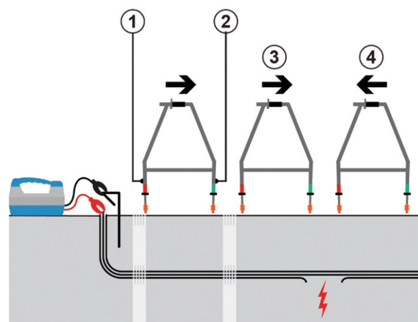
Figure 10.1: Cable sheath fault-finding
