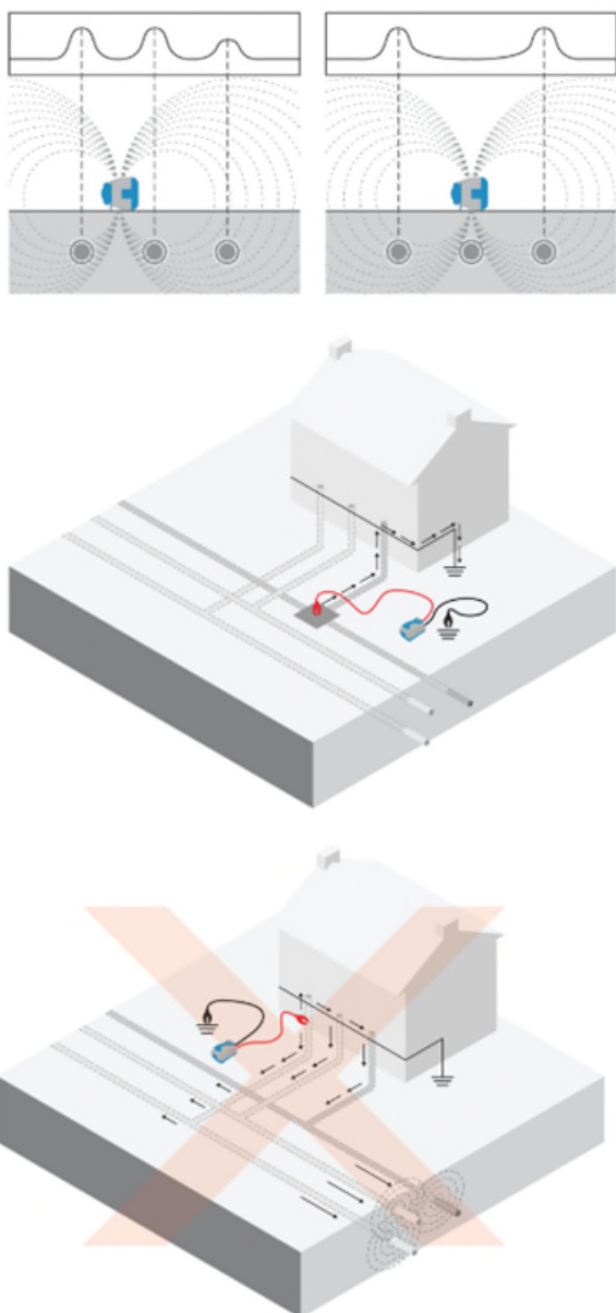
Figures 9.1 – 9.4: Nulling utilities & interference from services
