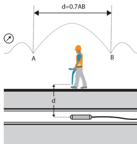
Figure 15.10: Calculating sonde depth
