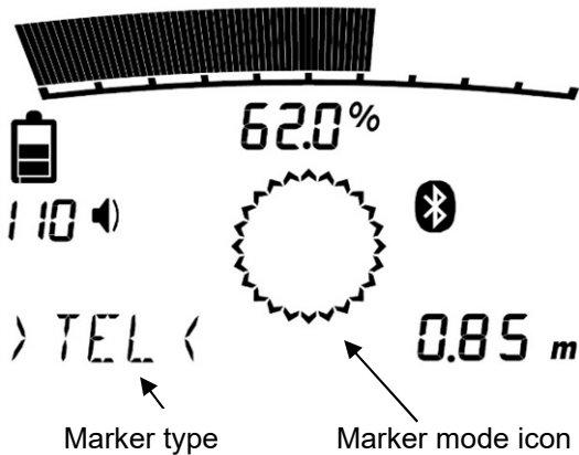
Figure 7.1 Marker mode
