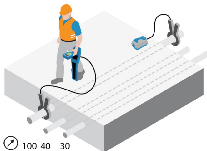
Figure 15.1: Connecting clamps
