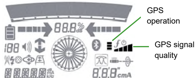
Figure 4.10 GPS Icons
