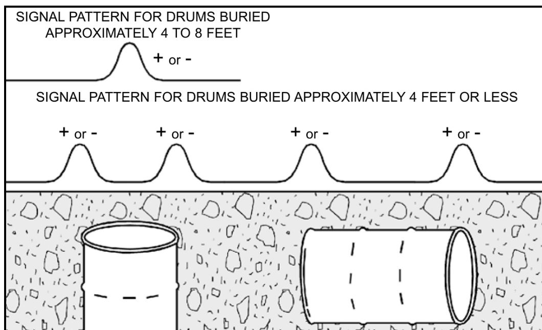
Figure 25: Signal Patterns provided by Steel Drums
